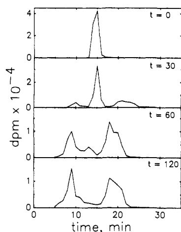
Figure 2. HPLC analysis of [^{14}\text{C}] -1 oxidation products. [^{14}\text{C}] -1 was incubated with AMVN in acetonitrile as described under the Experimental Section. Although the time scales are identical, the chromatograms are offset for clarity.
