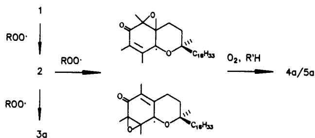
Figure 9. Proposed mechanisms for oxidation of 2 by peroxy radicals to 8a-(alkyldioxy)tocopherone 3a and epoxytocopherones 4a and 5a (see text for Discussion).
